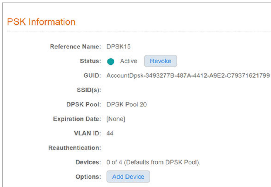
FIGURE 6 DPSK15 Information in UI After API PUT Call
